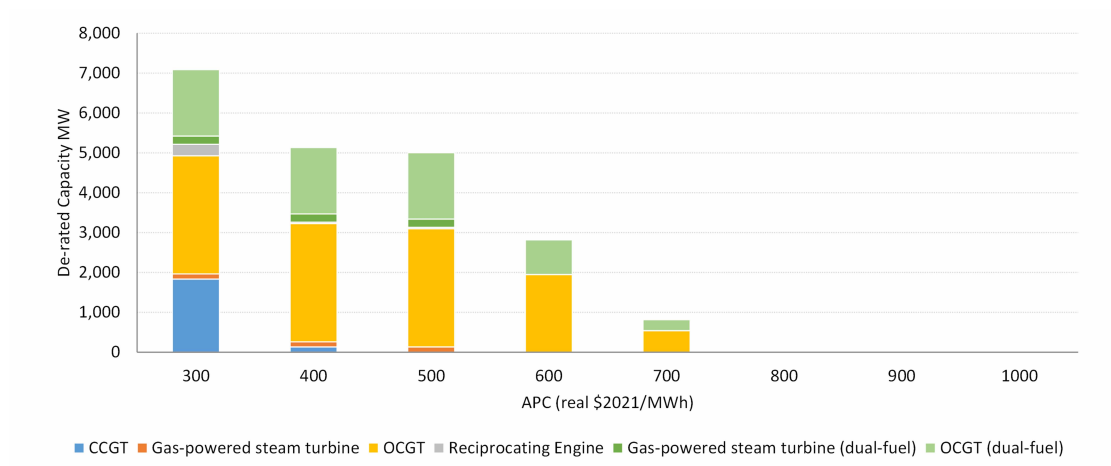
Figure 5.2: Supply stack thermal generation above $300/MWh - high price scenario
